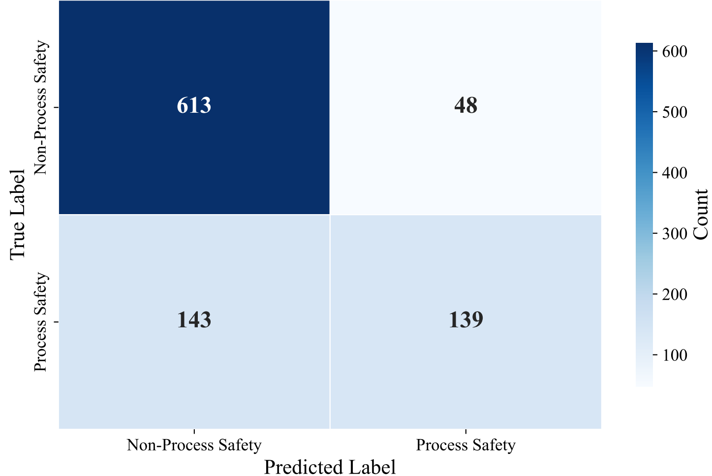
Confusion Matrix — ENGLISH_MANUAL (bert-base-multilingual-uncased, Random_Forest)
