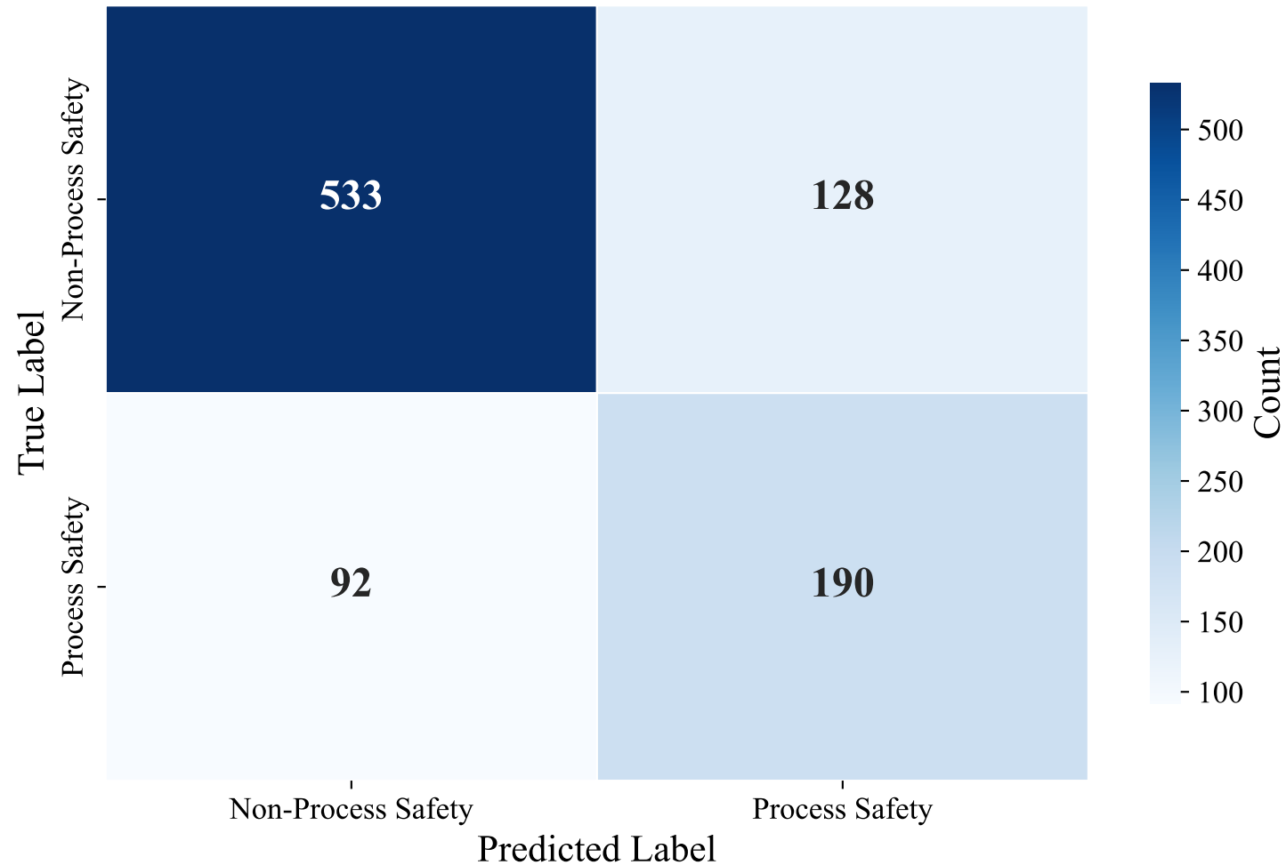
Confusion Matrix — ENGLISH_MANUAL (intfloat/multilingual-e5-large-instruct, SVM)
