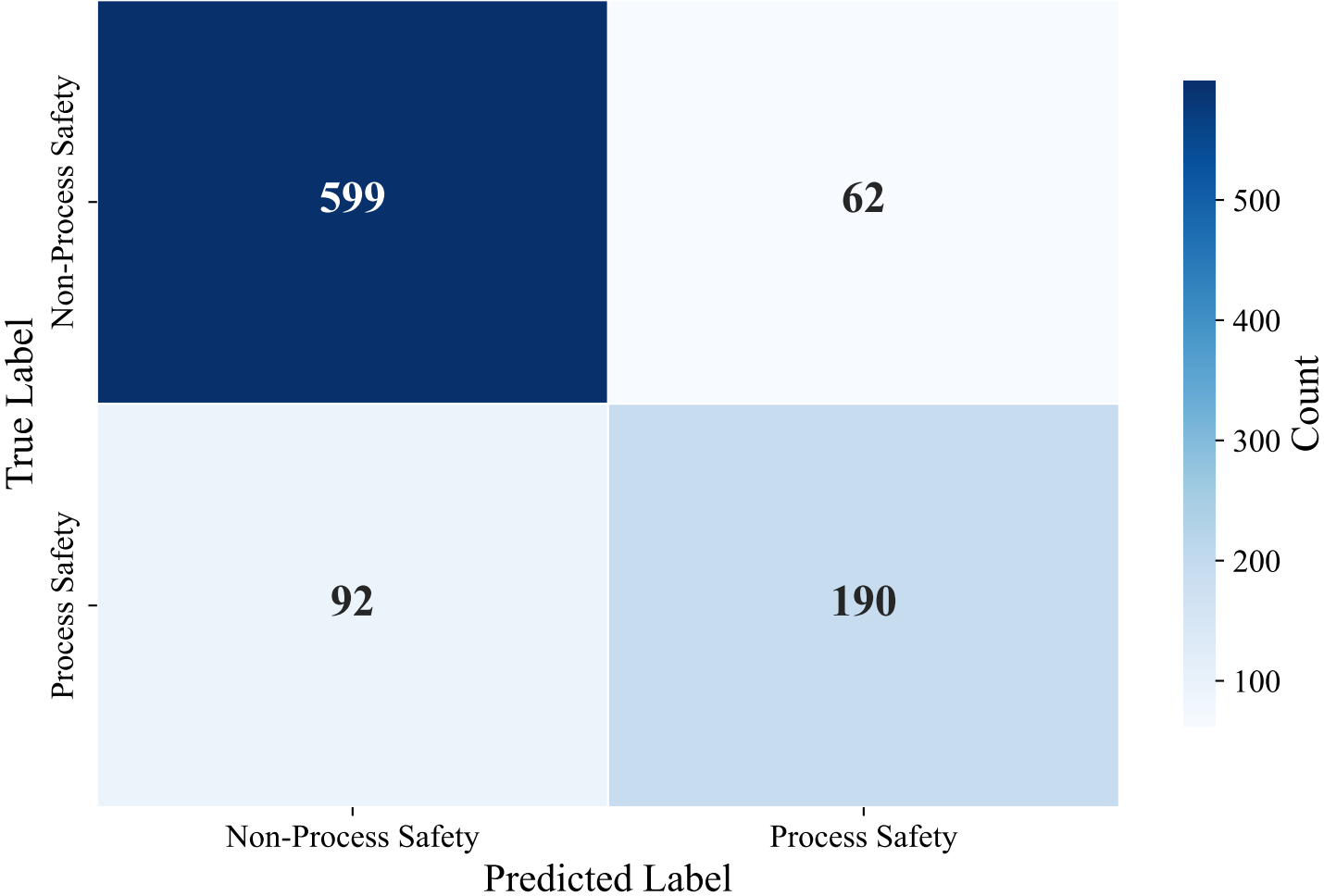
Confusion Matrix — ENGLISH_MANUAL (intfloat/multilingual-e5-large-instruct, Voting_Ensemble)
