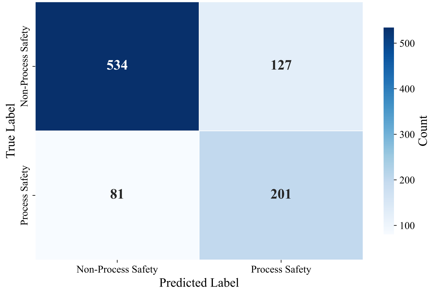
Confusion Matrix — ENGLISH_MANUAL (paraphrase-multilingual-MiniLM-L12-v2, SVM)
