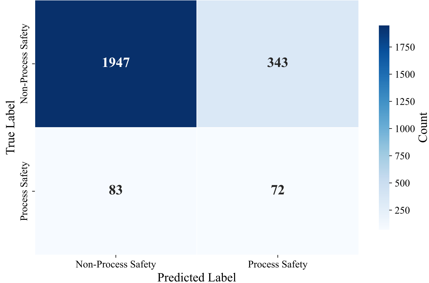
Confusion Matrix — SWEDISH_MANUAL (intfloat/multilingual-e5-large-instruct, SVM)
