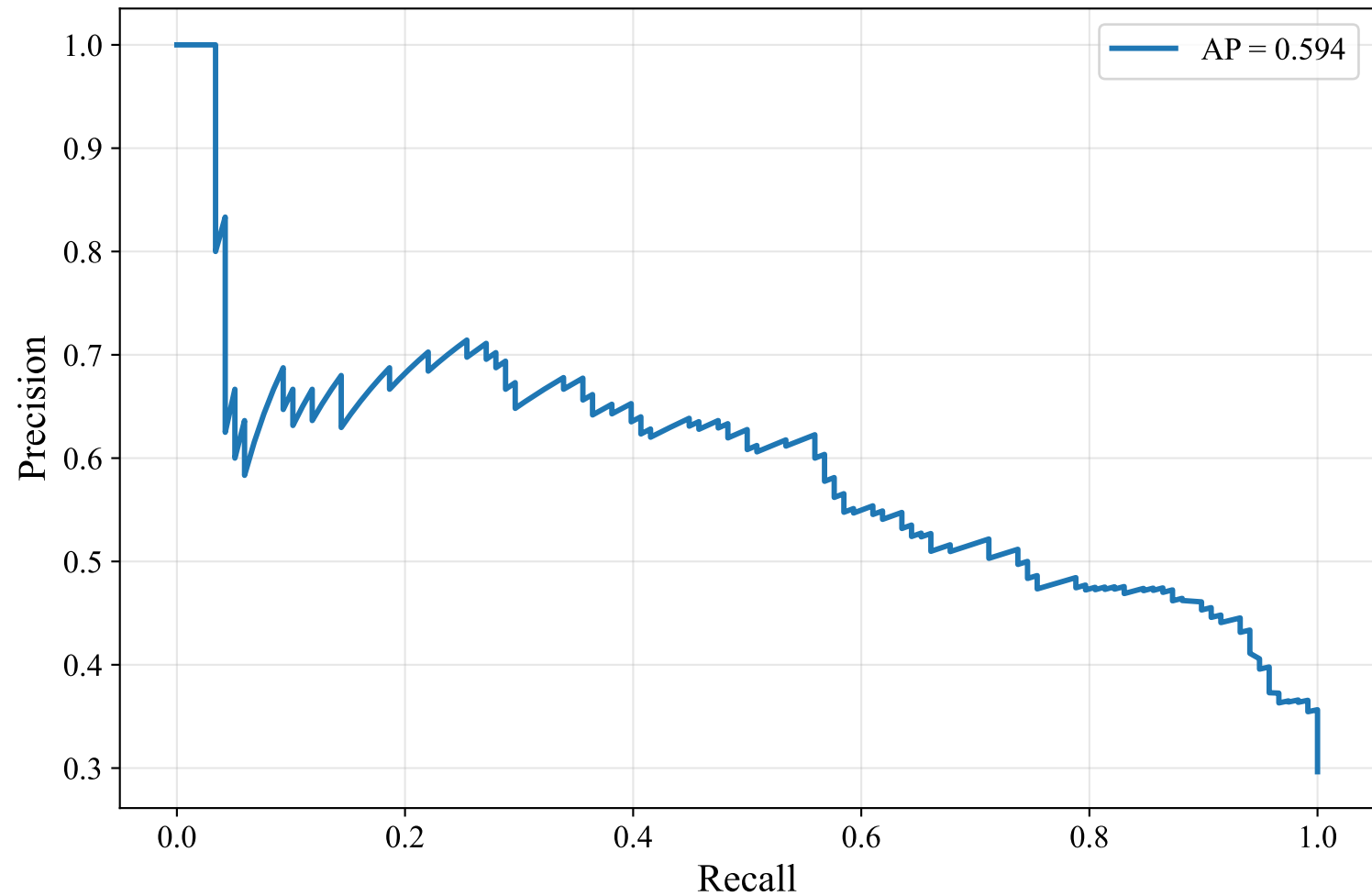
Precision-Recall Curve — DUTCH_MANUAL (paraphrase-multilingual-MiniLM-L12-v2, Random_Forest)
