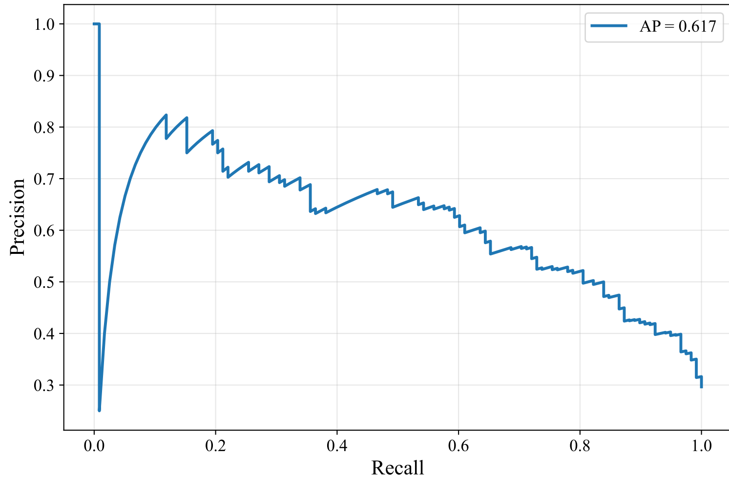
Precision-Recall Curve — DUTCH_MANUAL (xlm-roberta-base, LightGBM)
