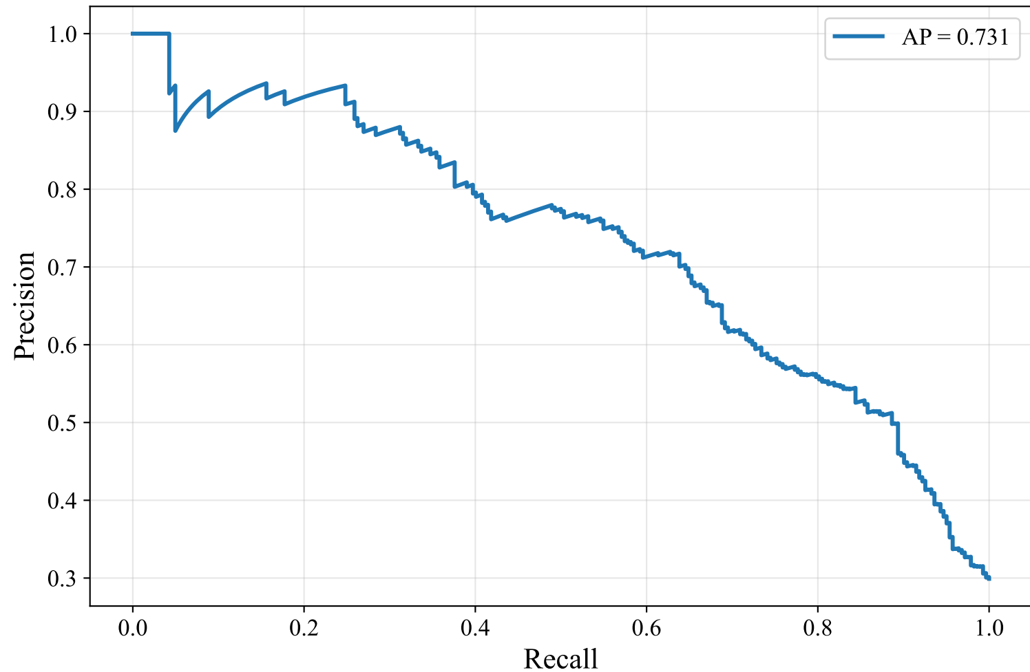
Precision-Recall Curve — ENGLISH_MANUAL (paraphrase-multilingual-MiniLM-L12-v2, SVM)
