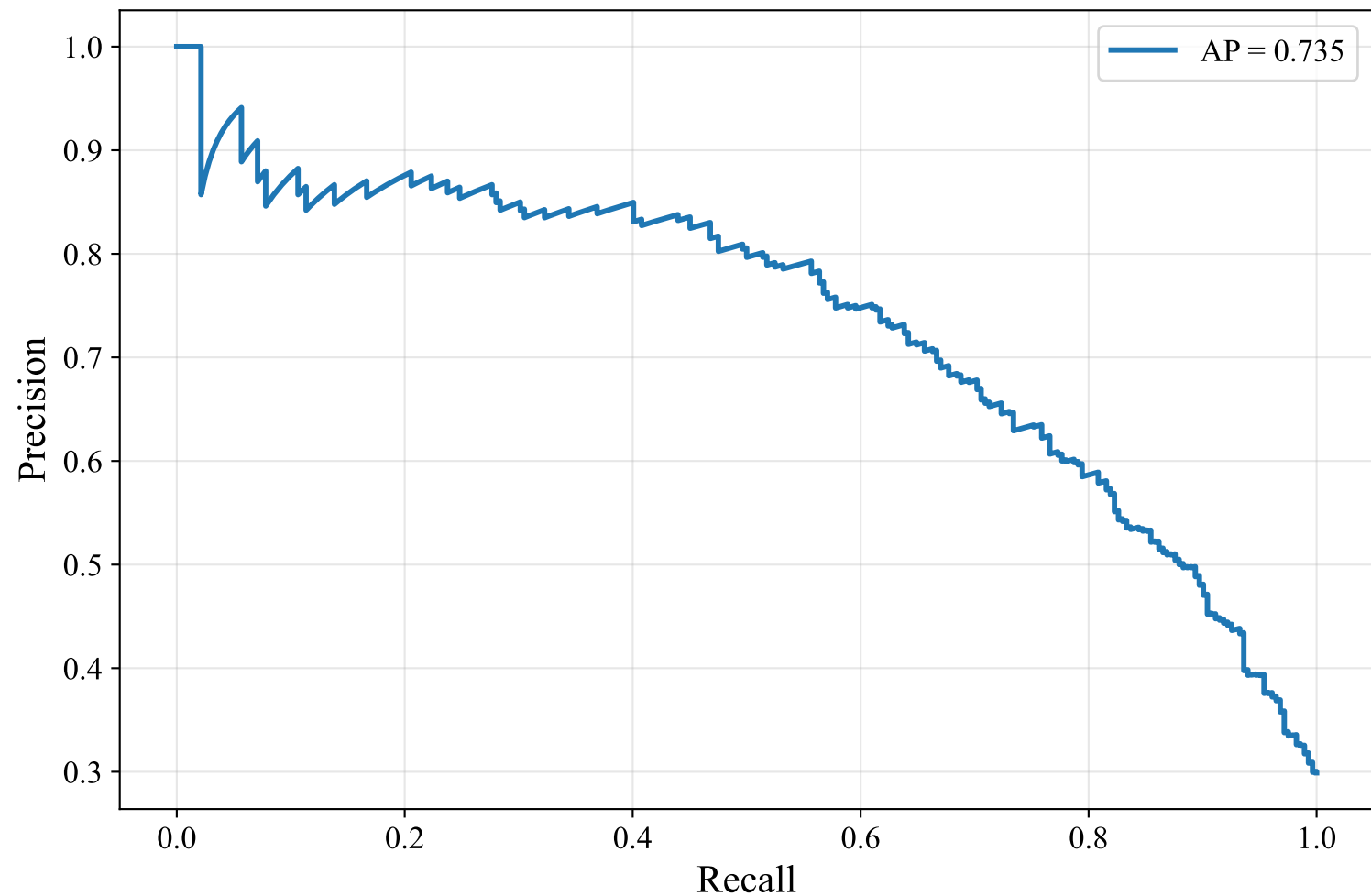
Precision-Recall Curve — ENGLISH_MANUAL (paraphrase-multilingual-MiniLM-L12-v2, XGBoost)
