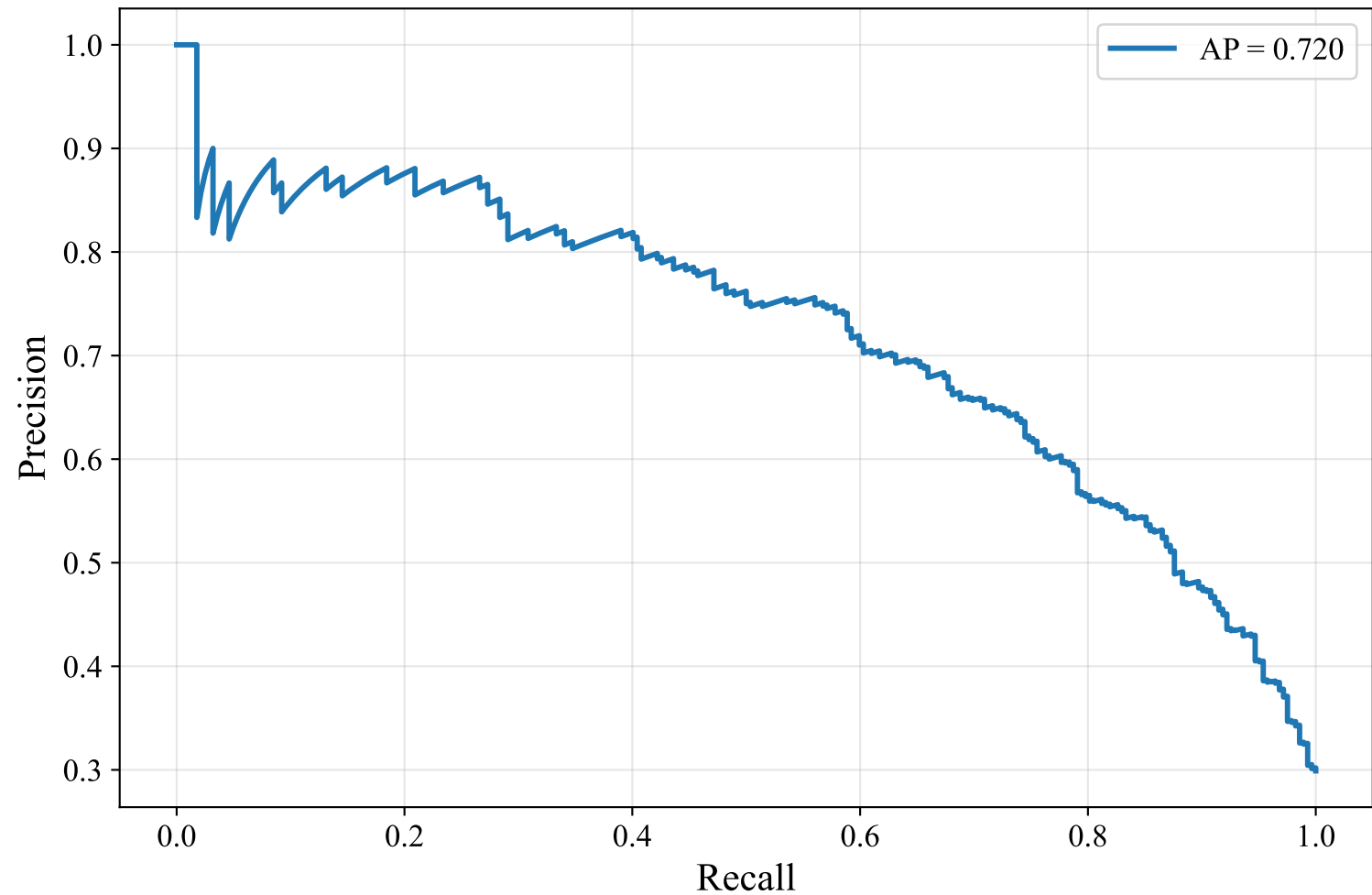
Precision-Recall Curve — ENGLISH_MANUAL (xlm-roberta-base, LightGBM)
