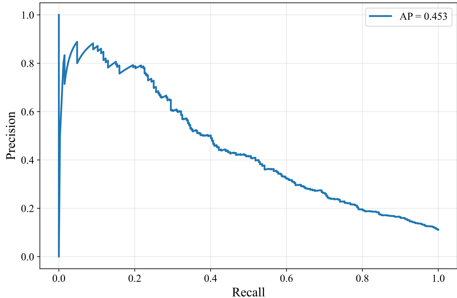
Precision-Recall Curve — GERMAN_MANUAL (Alibaba-NLP/gte-multilingual-base, LightGBM)
