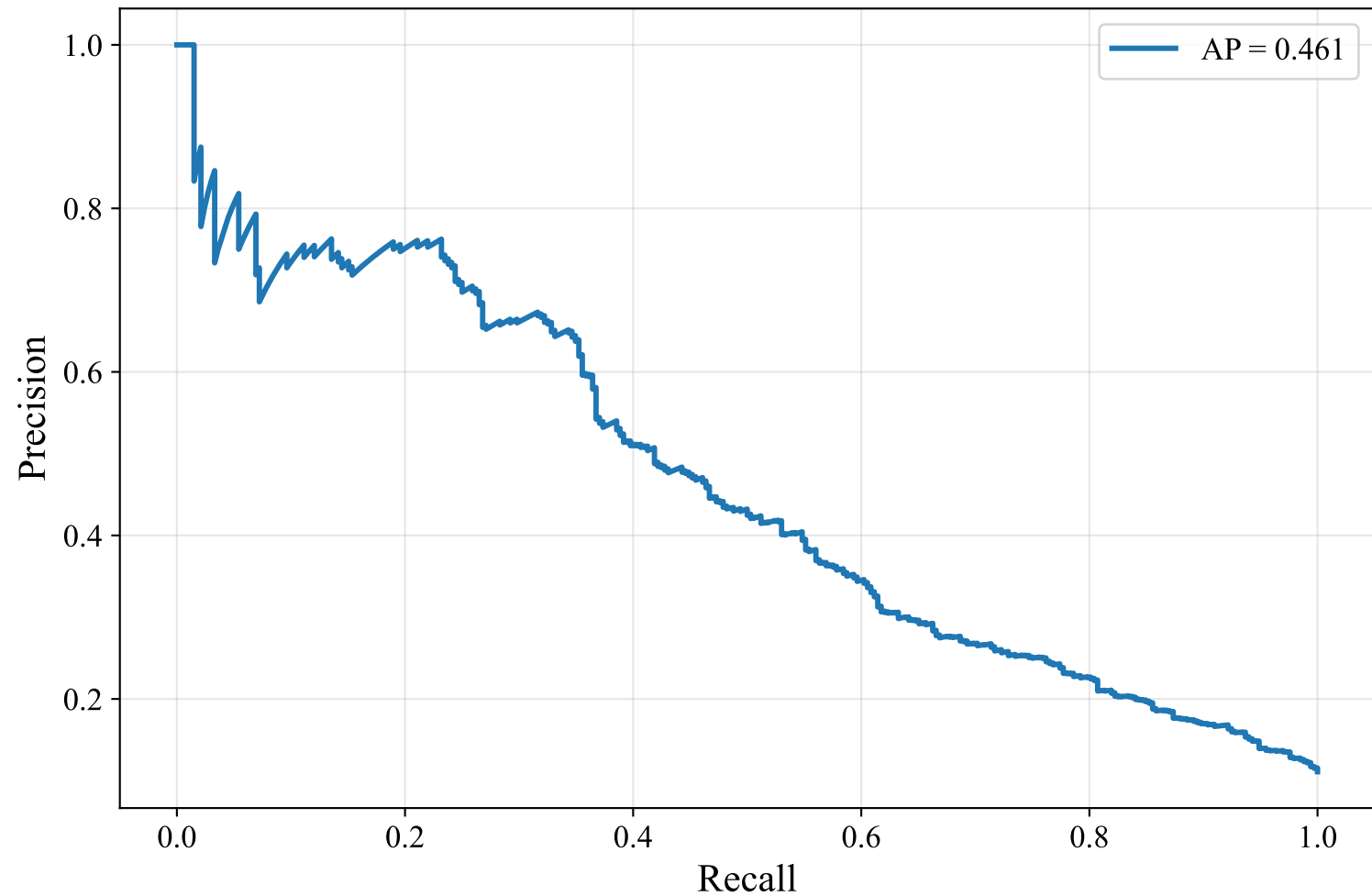
Precision-Recall Curve — GERMAN_MANUAL (bert-base-multilingual-uncased, LightGBM)
