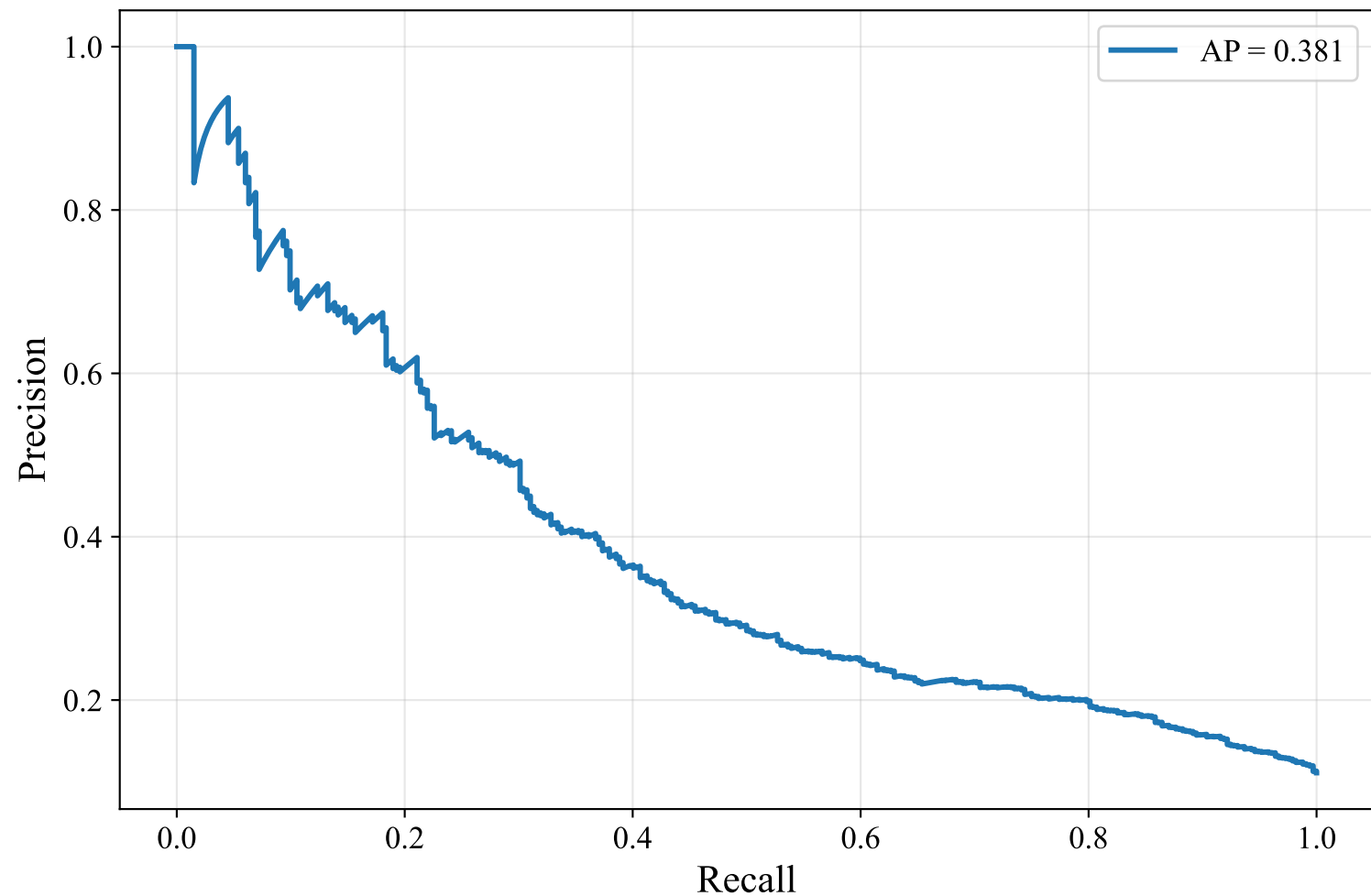
Precision-Recall Curve — GERMAN_MANUAL (paraphrase-multilingual-MiniLM-L12-v2, LightGBM)
