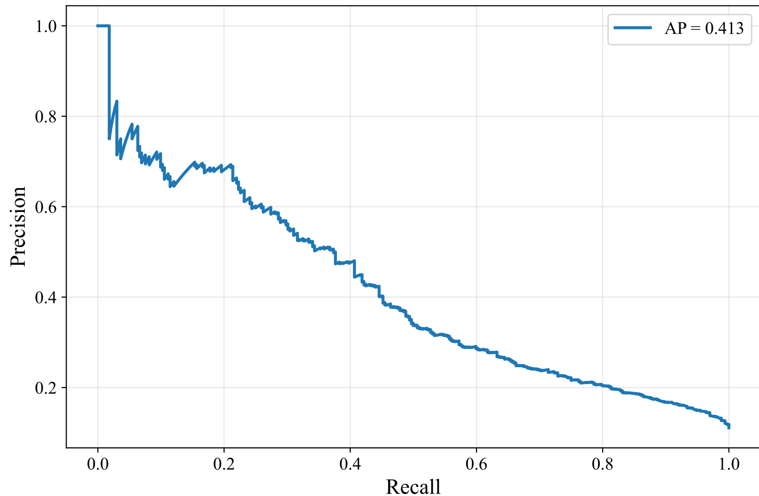
Precision-Recall Curve — GERMAN_MANUAL (paraphrase-multilingual-mpnet-base-v2, Random_Forest)
