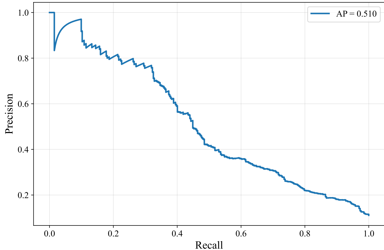
Precision-Recall Curve — GERMAN_MANUAL (upskyy/bge-m3-korean, XGBoost)
