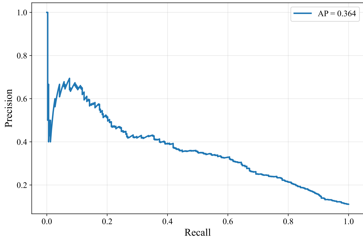
Precision-Recall Curve — GERMAN_MANUAL (xlm-roberta-base, SVM)
