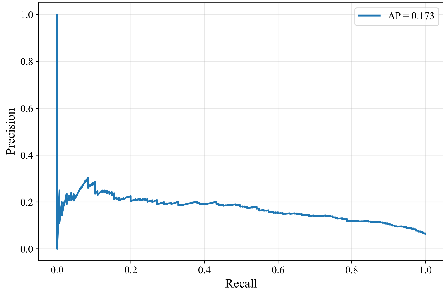
Precision-Recall Curve — SWEDISH_MANUAL (bert-base-multilingual-uncased, Random_Forest)
