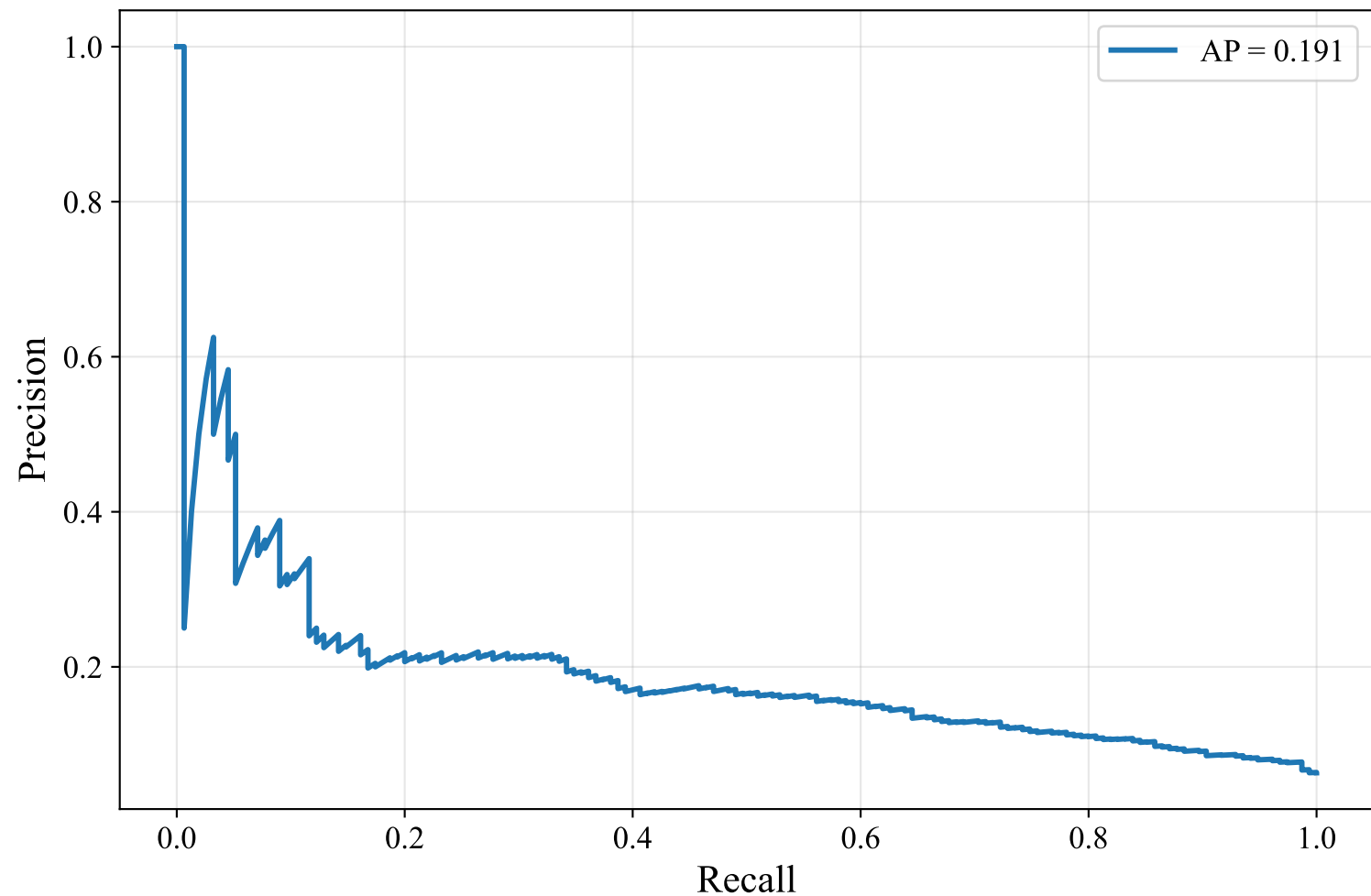
Precision-Recall Curve — SWEDISH_MANUAL (intfloat/multilingual-e5-large-instruct, SVM)
