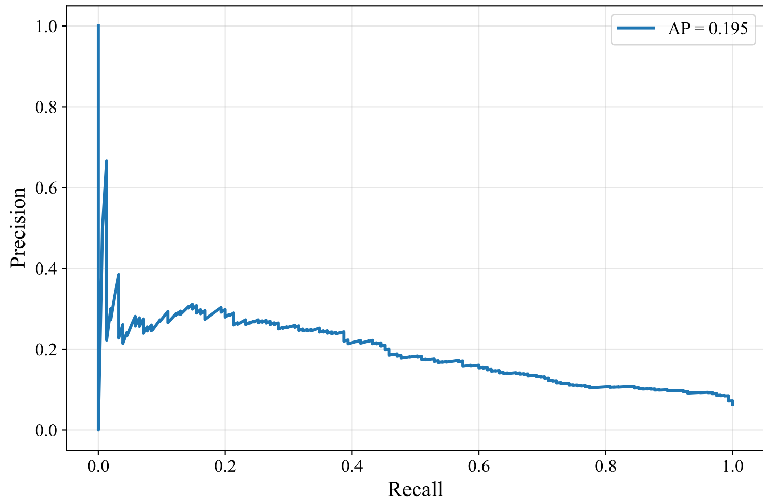
Precision-Recall Curve — SWEDISH_MANUAL (paraphrase-multilingual-MiniLM-L12-v2, LightGBM)
