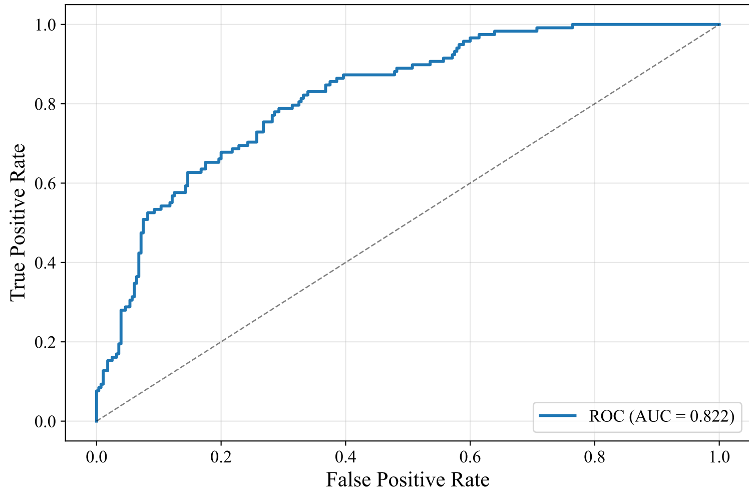
ROC Curve — DUTCH MANUAL (Alibaba-NLP/gte-multilingual-base, LightGBM)
