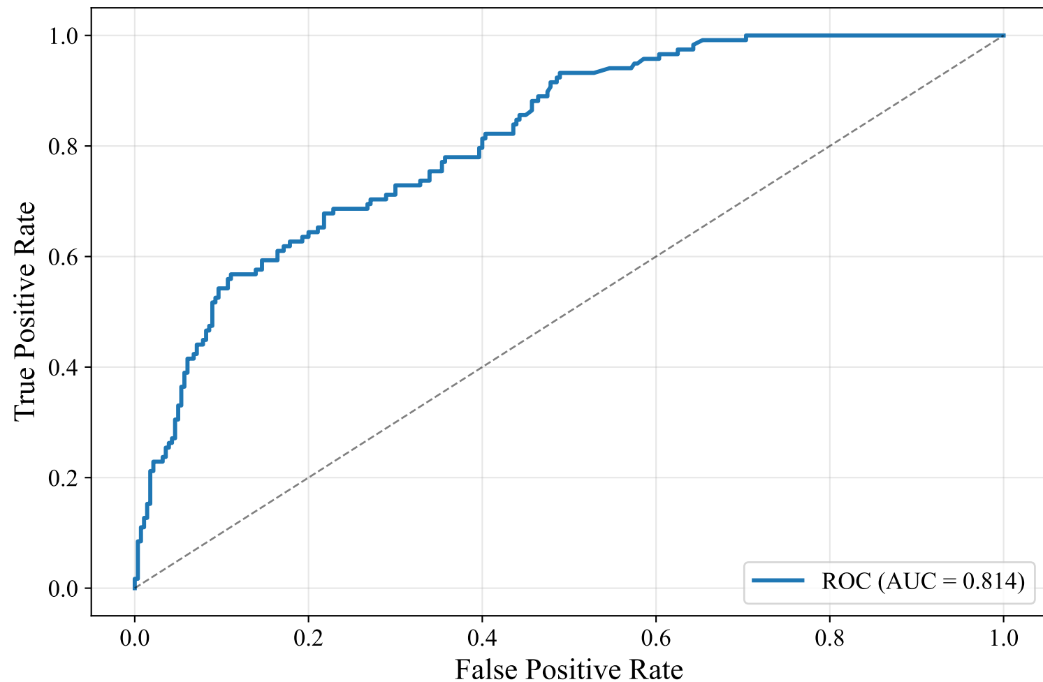
ROC Curve — DUTCH_MANUAL (Alibaba-NLP/gte-multilingual-base, Random_Forest)
