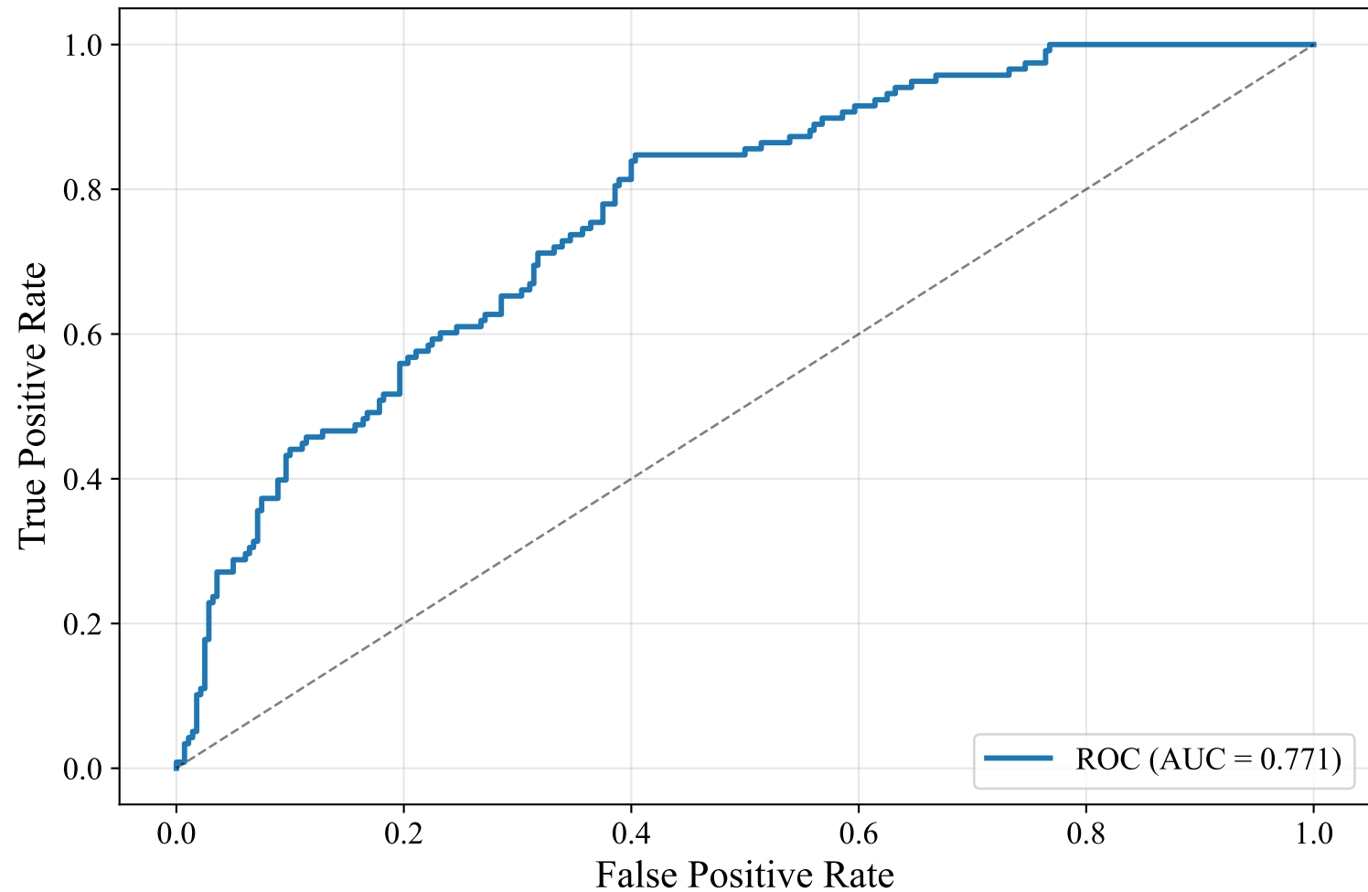
ROC Curve — DUTCH MANUAL (paraphrase-multilingual-MiniLM-L12-v2, LightGBM)
