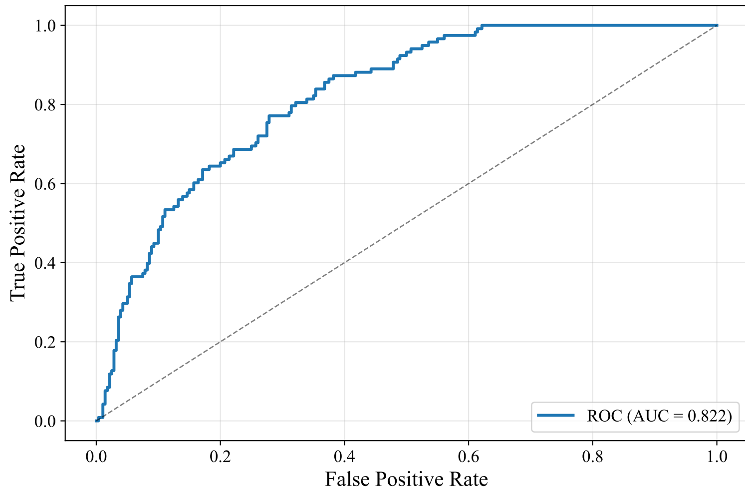
ROC Curve — DUTCH_MANUAL (snowflake-arctic-embed-l-v2.0, Random_Forest)
