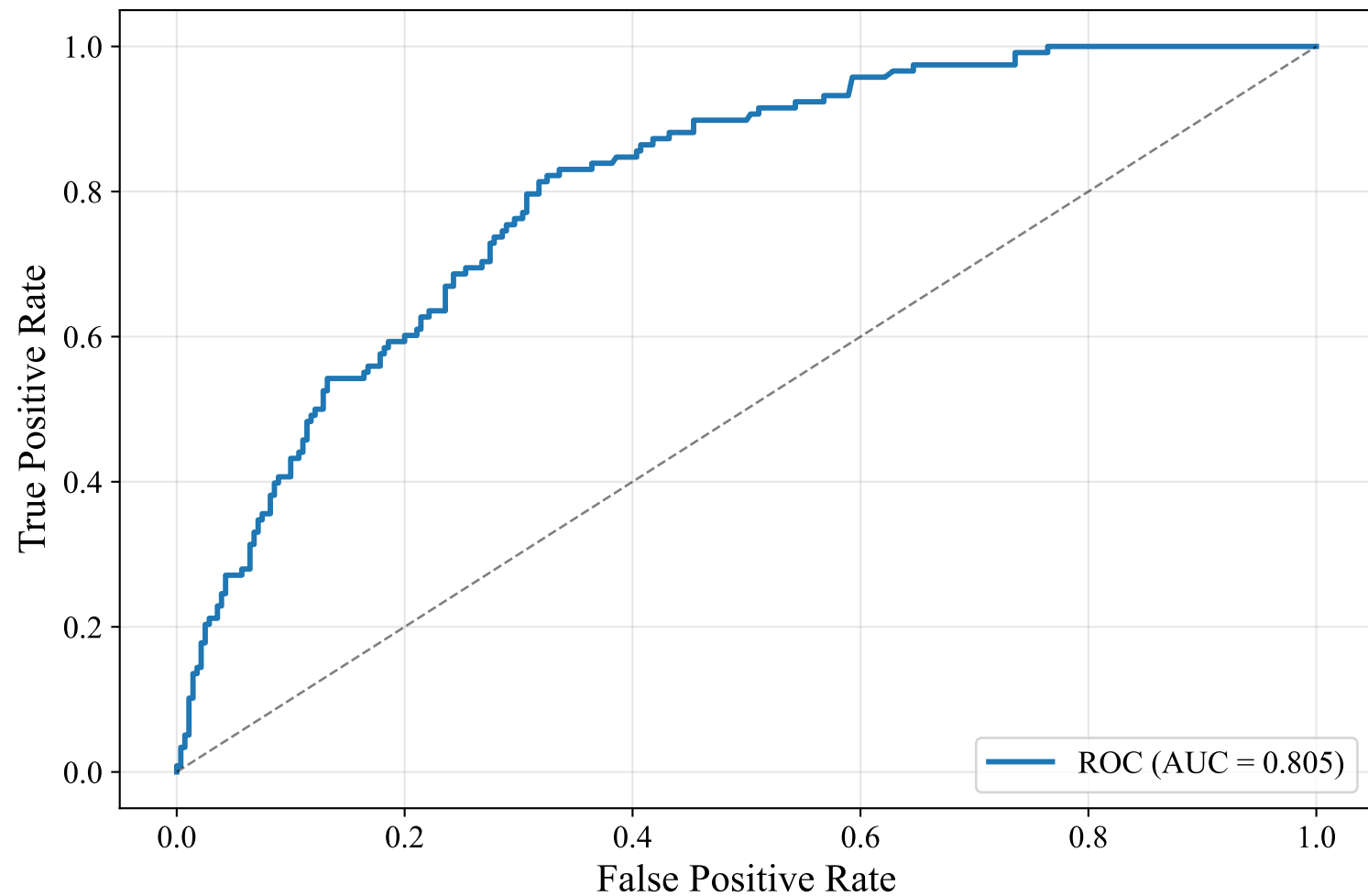
ROC Curve — DUTCH_MANUAL (upskyy/bge-m3-korean, Random_Forest)
