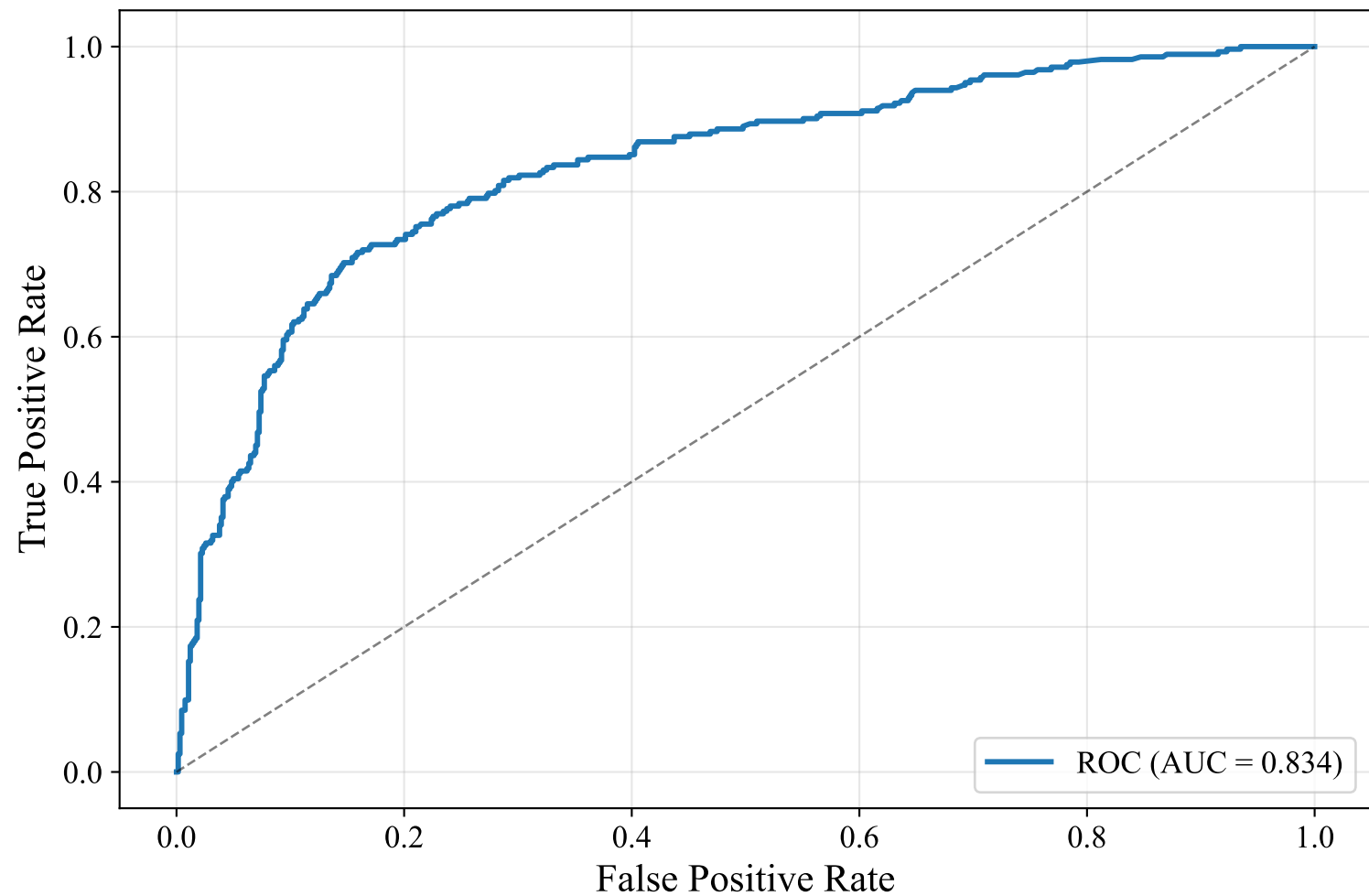
ROC Curve — ENGLISH_MANUAL (bert-base-multilingual-uncased, Random_Forest)
