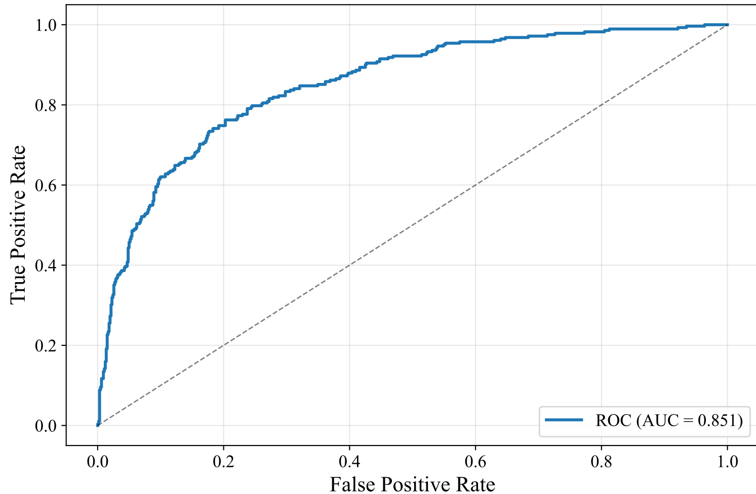
ROC Curve — ENGLISH_MANUAL (bert-base-multilingual-uncased, XGBoost)
