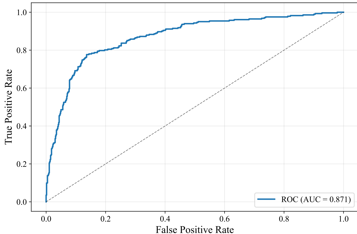
ROC Curve — ENGLISH_MANUAL (snowflake-arctic-embed-l-v2.0, XGBoost)
