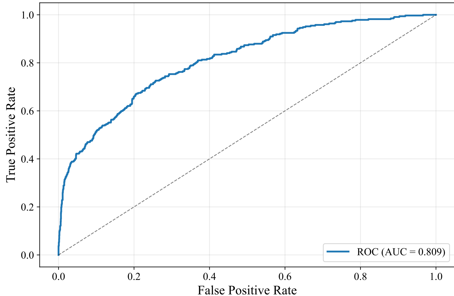
ROC Curve — GERMAN_MANUAL (Alibaba-NLP/gte-multilingual-base, XGBoost)
