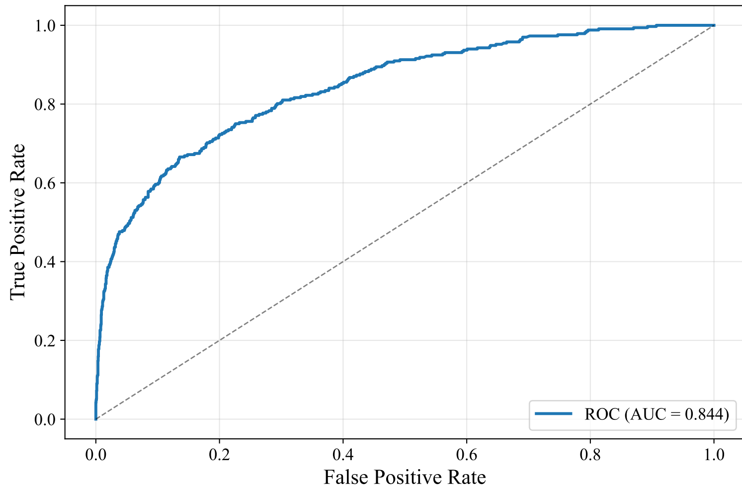
ROC Curve — GERMAN_MANUAL (intfloat/multilingual-e5-large-instruct, Random_Forest)
