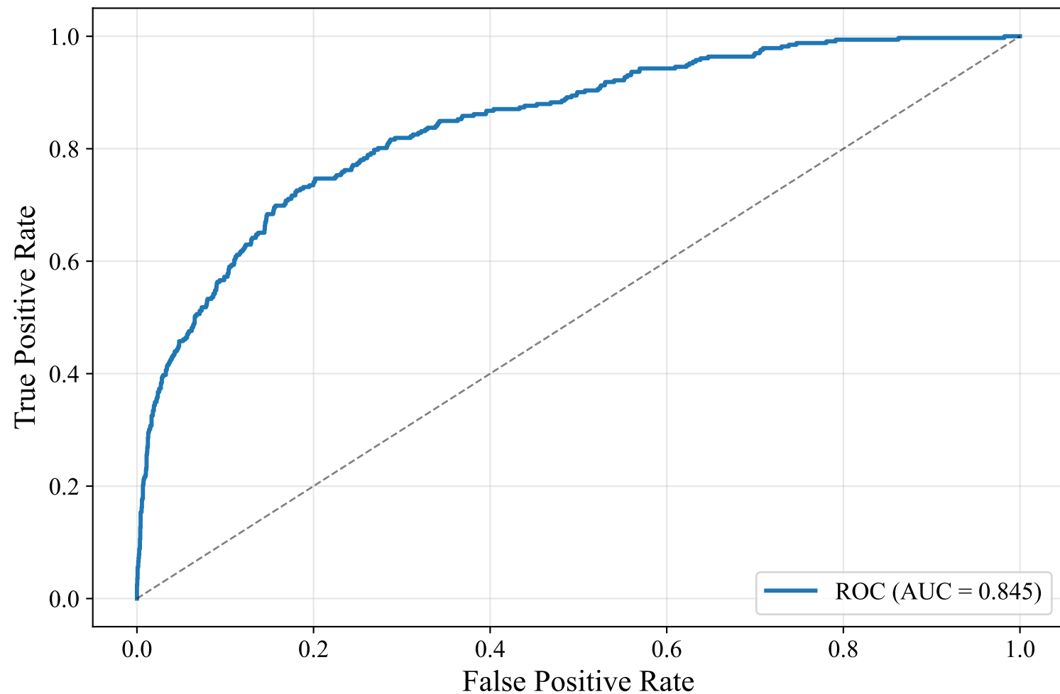
ROC Curve — GERMAN_MANUAL (snowflake-arctic-embed-l-v2.0, XGBoost)
