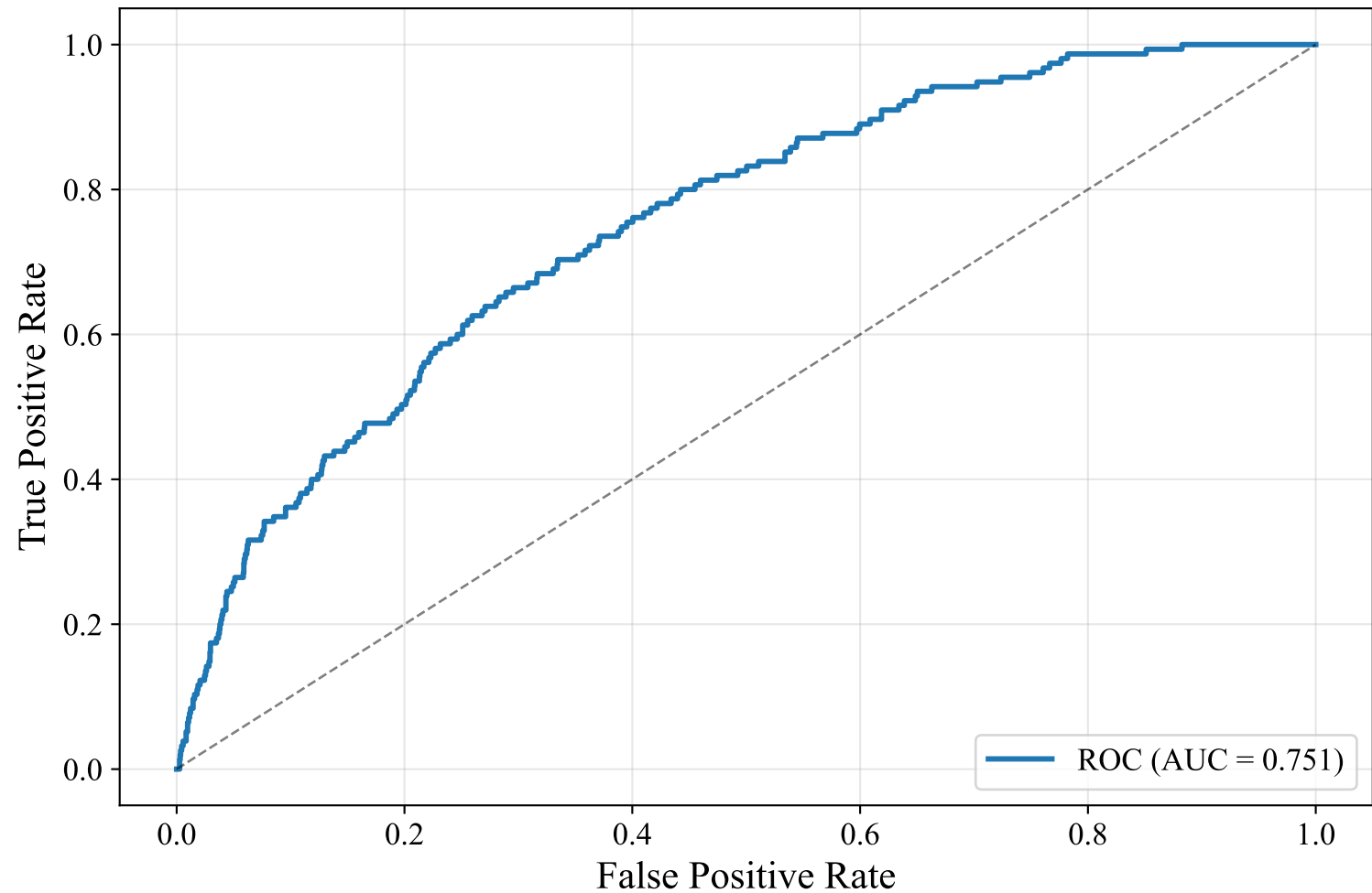
ROC Curve — SWEDEN_MANUAL (bert-base-multilingual-uncased, XGBoost)
