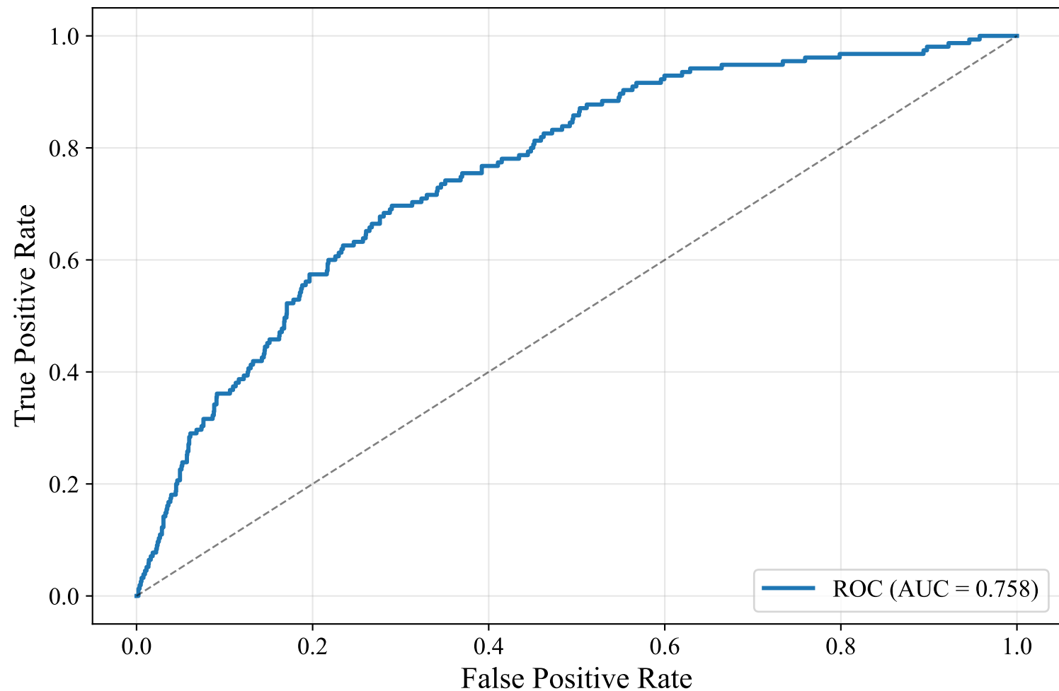
ROC Curve — SWEDISH_MANUAL (bert-base-multilingual-uncased, LightGBM)
