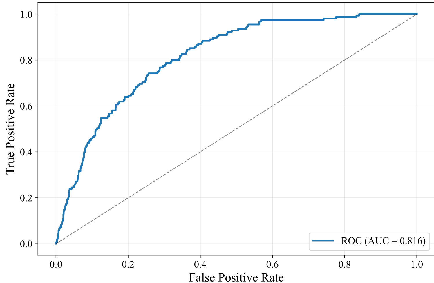
ROC Curve — SWEDISH_MANUAL (intfloat/multilingual-e5-large-instruct, XGBoost)
