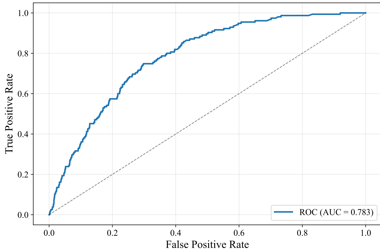
ROC Curve — SWEDISH_MANUAL (paraphrase-multilingual-mpnet-base-v2, Random_Forest)
