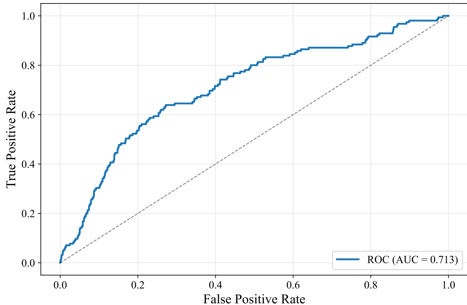
ROC Curve — SWEDISH_MANUAL (paraphrase-multilingual-mpnet-base-v2, SVM)
