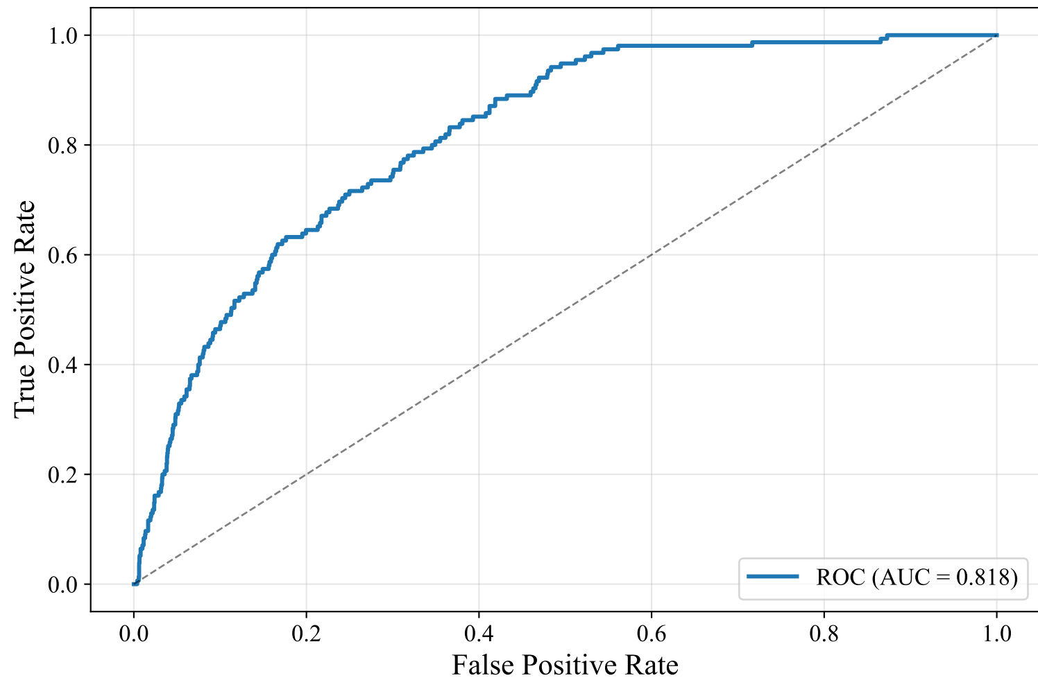
ROC Curve — SWEDISH_MANUAL (snowflake-arctic-embed-l-v2.0, Random_Forest)
