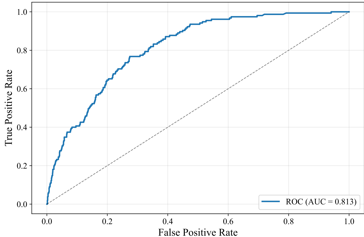
ROC Curve — SWEDISH_MANUAL (upskyy/bge-m3-korean, Random_Forest)
