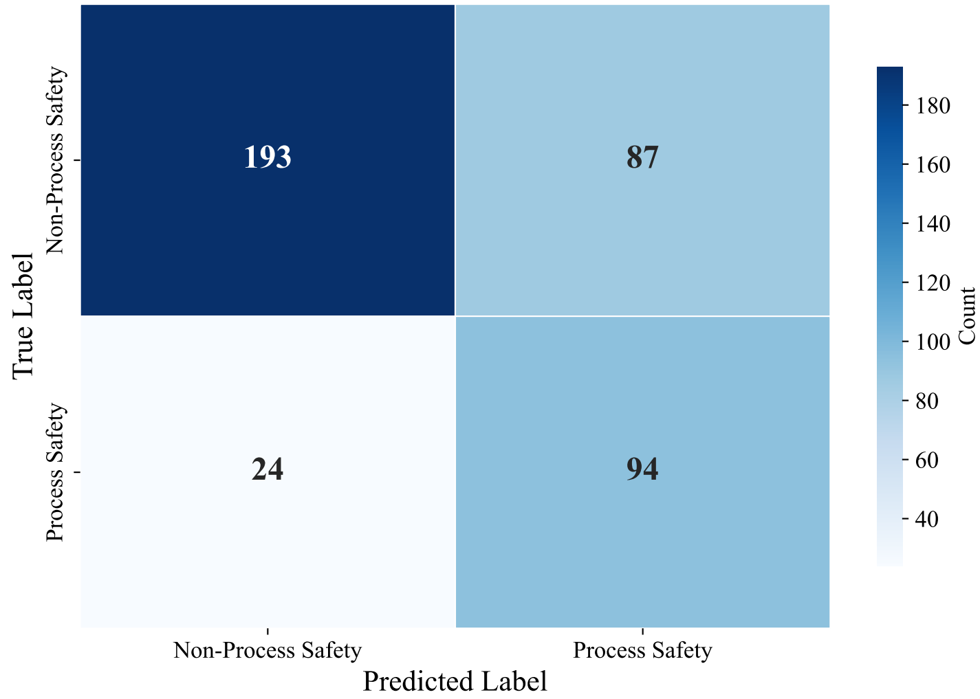
Confusion Matrix — DUTCH_MANUAL (efederici/e5-base-multilingual-4096, Voting_Ensemble)
