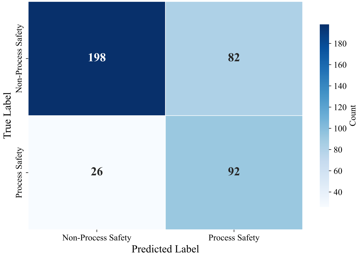
Confusion Matrix — DUTCH_MANUAL (efederici/e5-base-multilingual-4096, XGBoost_Optimized)
