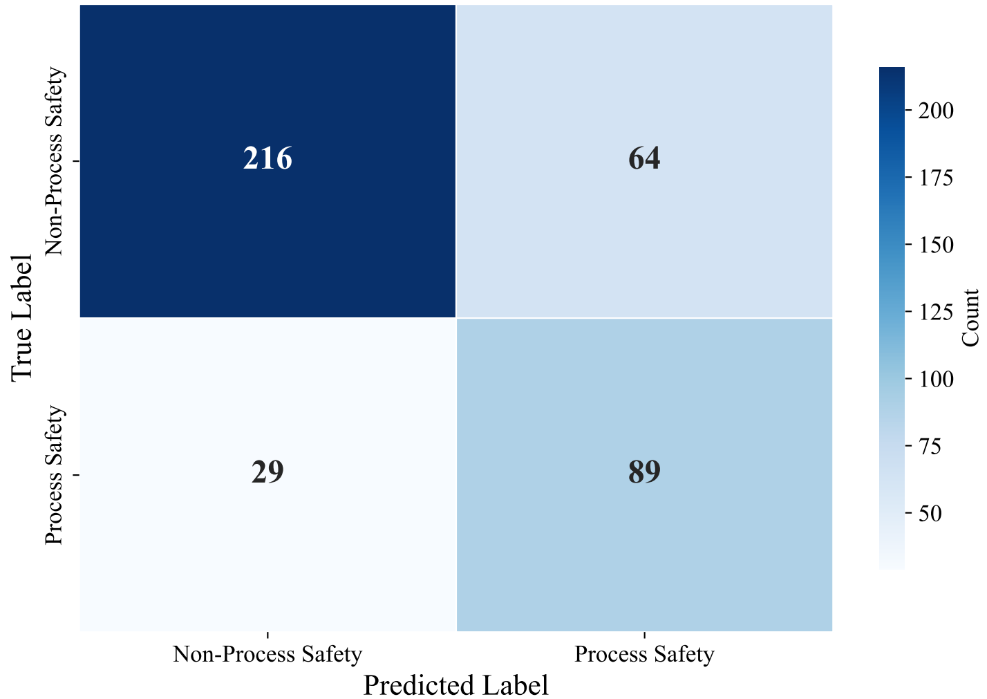
Confusion Matrix — DUTCH_MANUAL (intfloat/multilingual-e5-large-instruct, LightGBM_Optimized)
