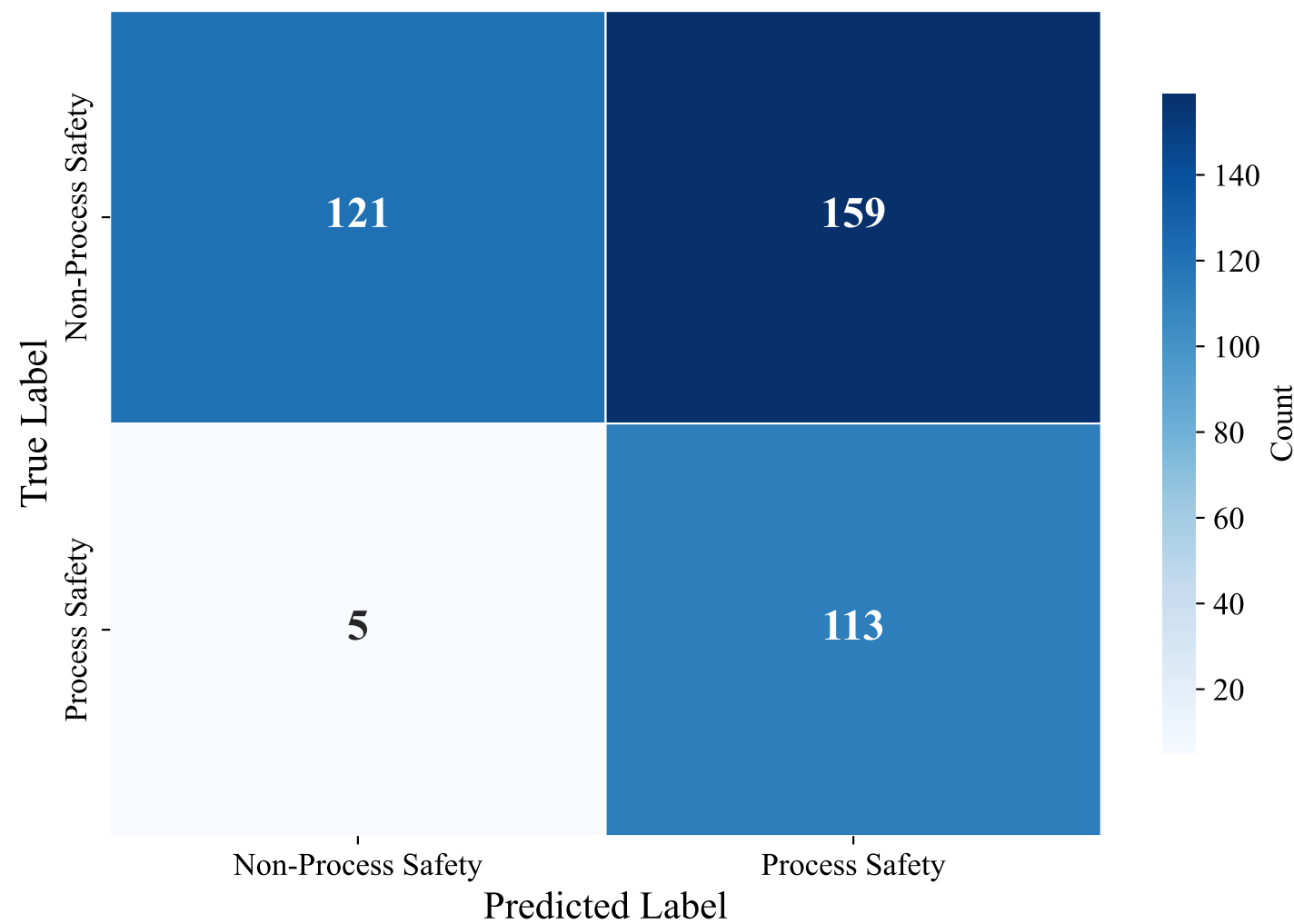
Confusion Matrix — DUTCH_MANUAL (intfloat/multilingual-e5-large-instruct, Random_Forest_Optimized)
