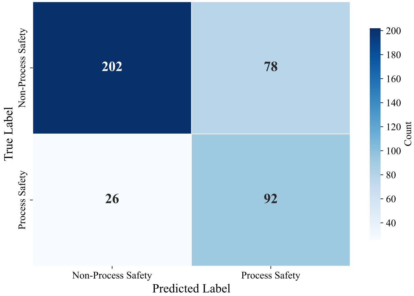
Confusion Matrix — DUTCH_MANUAL (intfloat/multilingual-e5-large-instruct, XGBoost_Optimized)
