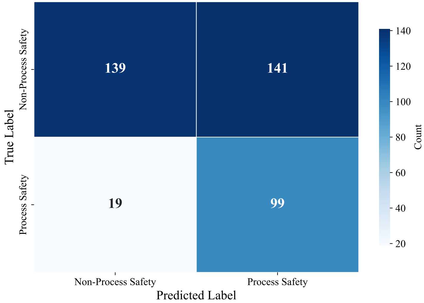
Confusion Matrix — DUTCH_MANUAL (upskyy/bge-m3-korean, Random_Forest)
