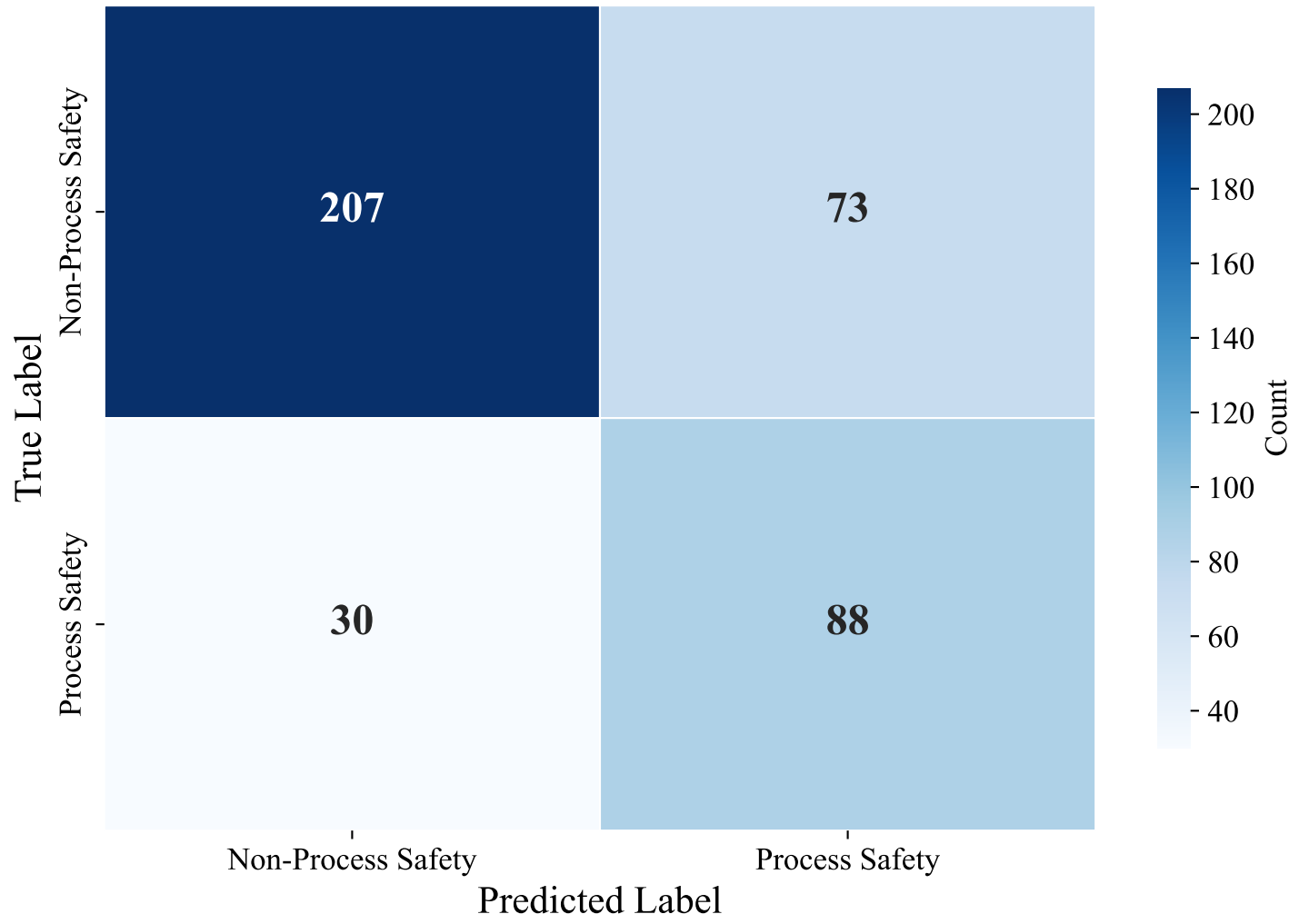
Confusion Matrix — DUTCH_MANUAL (upskyy/bge-m3-korean, XGBoost_Optimized)
