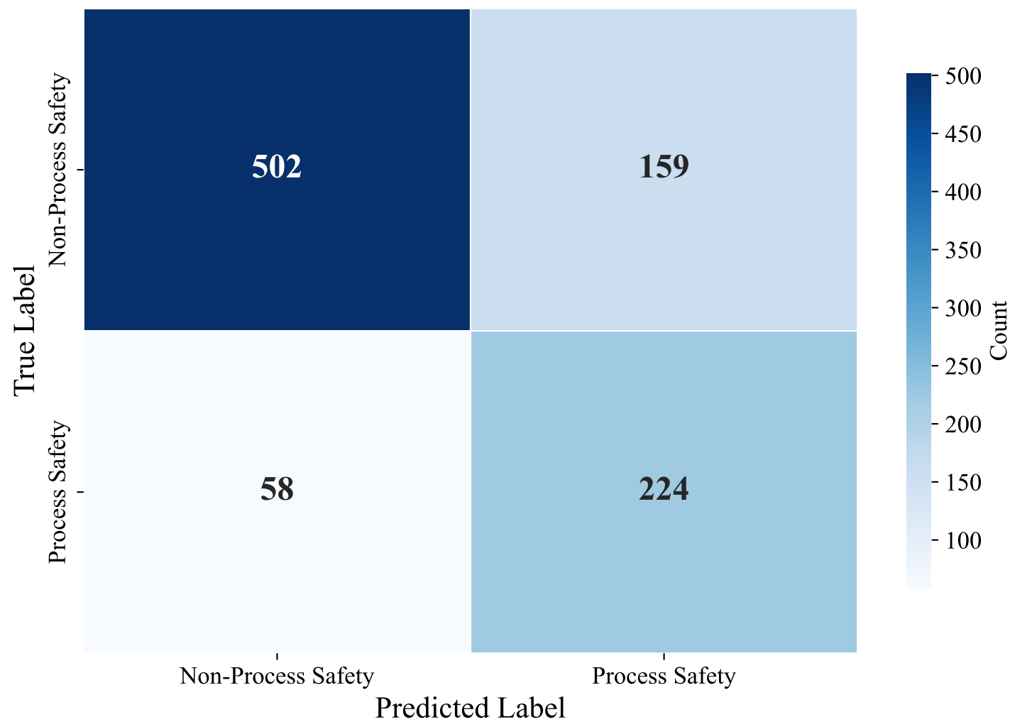
Confusion Matrix — ENGLISH_MANUAL (efederici/e5-base-multilingual-4096, LightGBM)
