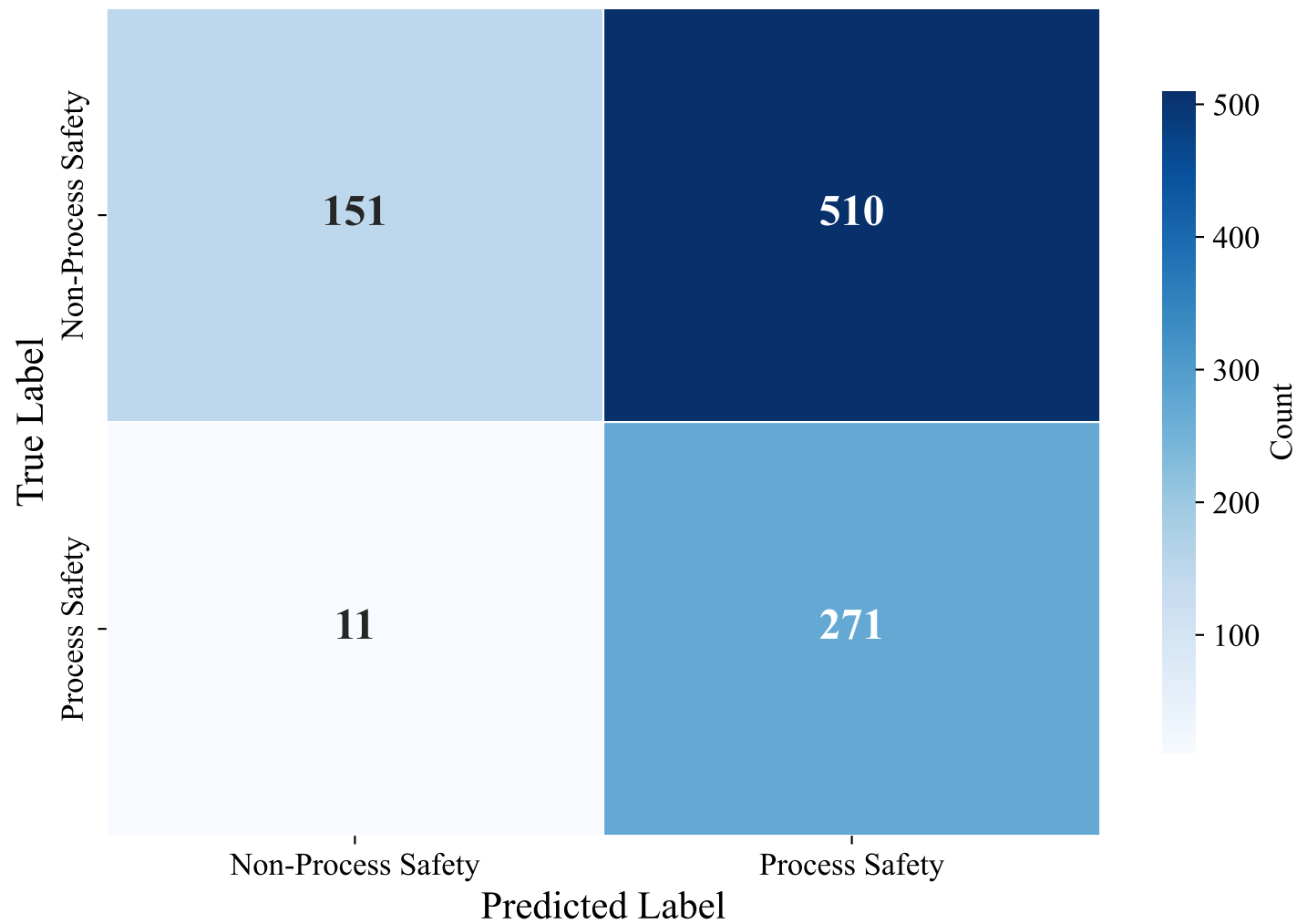
Confusion Matrix — ENGLISH_MANUAL (intfloat/multilingual-e5-large-instruct, Random_Forest_Optimized)
