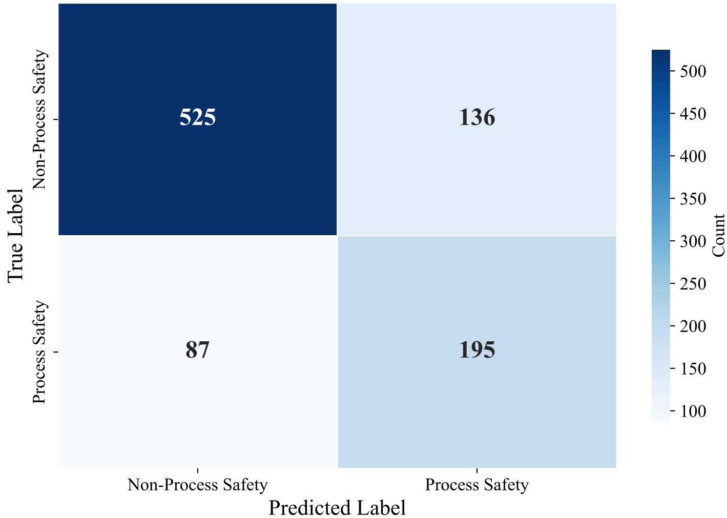
Confusion Matrix — ENGLISH_MANUAL (intfloat/multilingual-e5-large-instruct, SVM)
