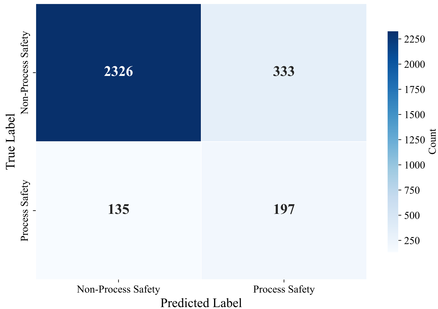
Confusion Matrix — GERMAN_MANUAL (efederici/e5-base-multilingual-4096, LightGBM)
