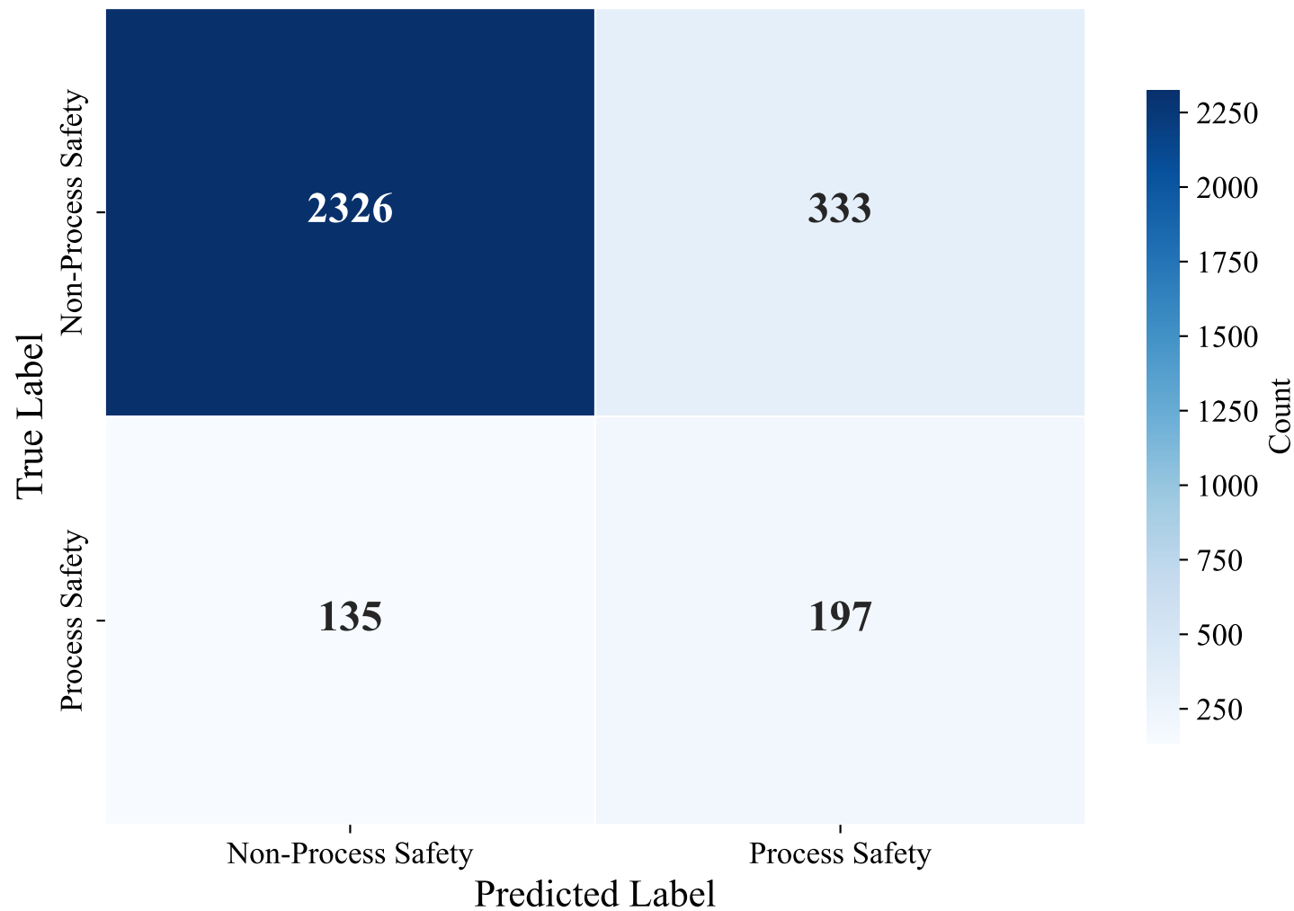
Confusion Matrix — GERMAN_MANUAL (efederici/e5-base-multilingual-4096, LightGBM_Optimized)
