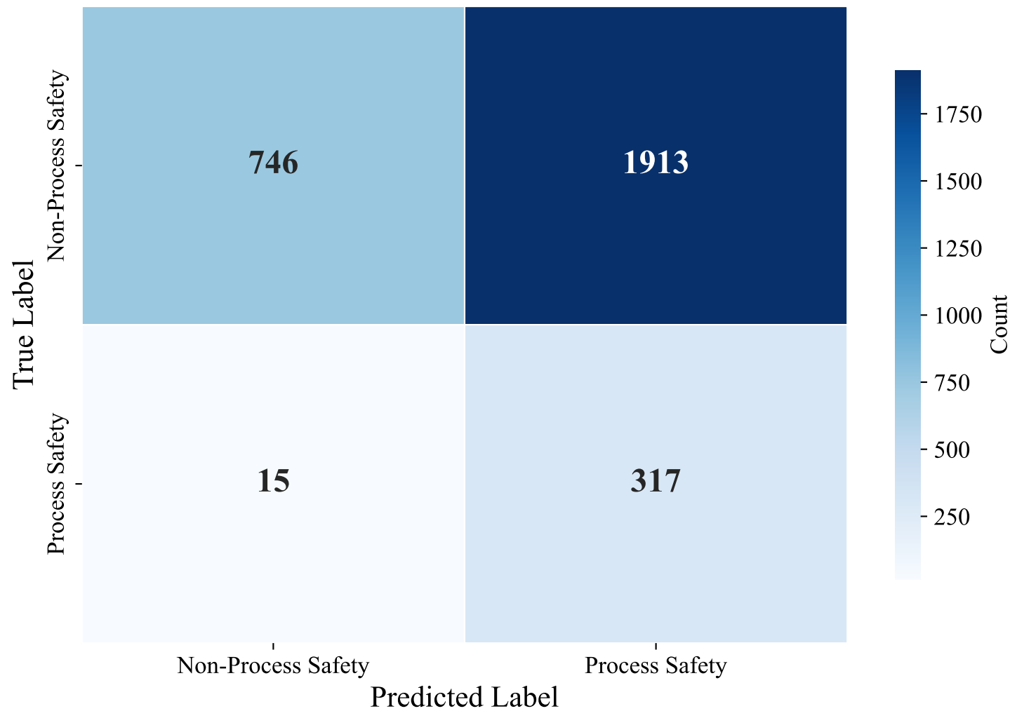
Confusion Matrix — GERMAN_MANUAL (intfloat/multilingual-e5-large-instruct, Random_Forest_Optimized)
